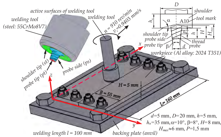
Fig. 1. rinciple of the FSW, welding tool and active surfaces of the welding tool
