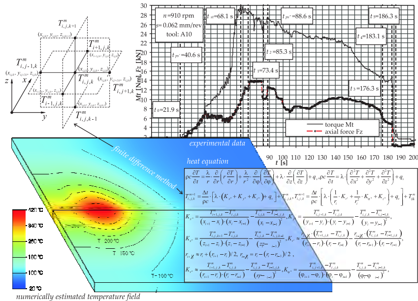
Fig. 3. Numerical simulation of the FSW
