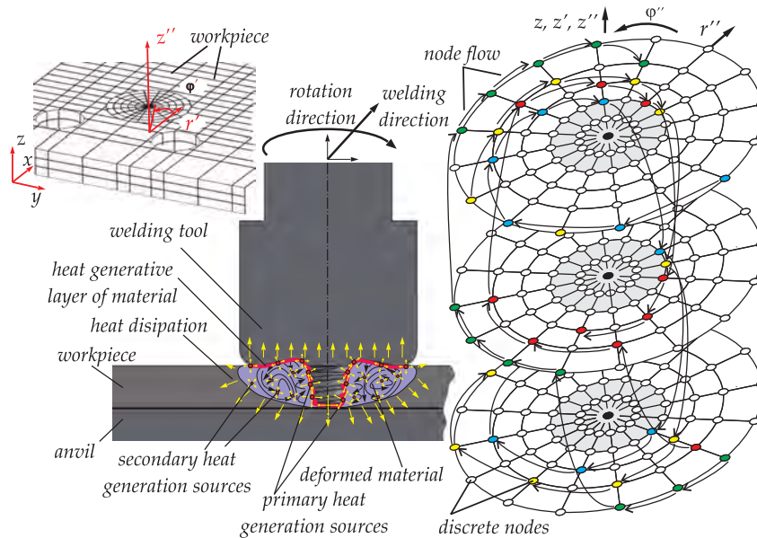
Fig. 2. pace discretization, heat generation and material flow pattern - node substitution and replacement during FSW
